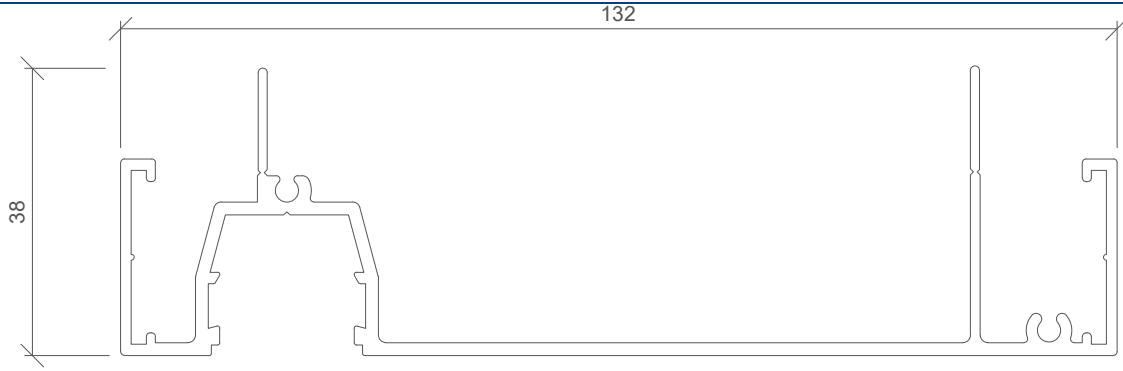
EDGE GLAZED POCKET HEADSECTION PSL 818
