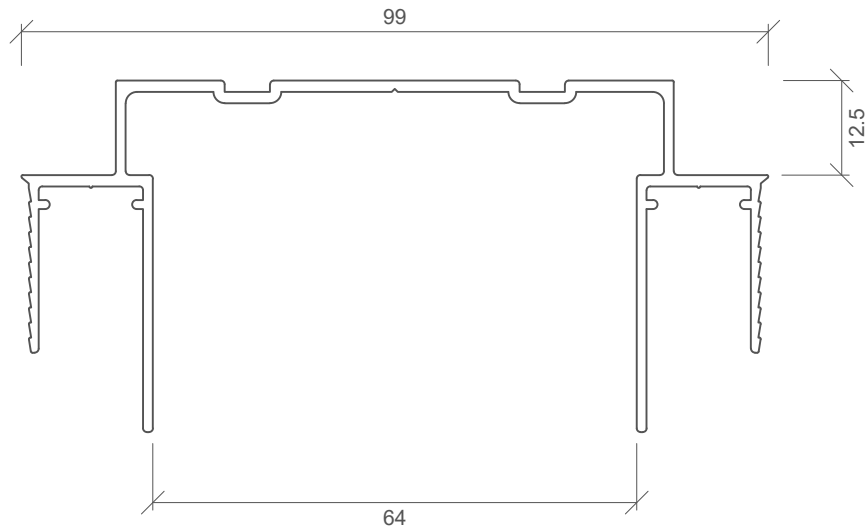
NEGATIVE DETAIL HEADSECTION - 64mm STUD/13mm LININGS PSL 740
