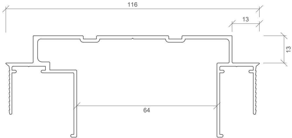
64mm NEGATIVE DETAIL HEAD TRACK THREE LAYERS 13mm PLASTERBOARD PSL 757
