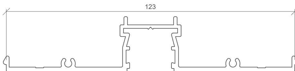
92mm POCKET STARTER FOUR LAYERS 13mm PLASTERBOARD PSL 892
