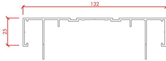
92mm GROOVED HEADSECTION PSL 420
