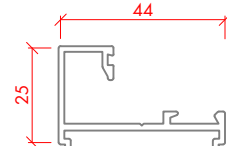
GLAZING BAR WITH LEGS (GLAZING BAR 2) PSL 210
