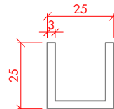
25 X 25 X 3 CHANNEL PSL 320
