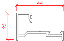
GLAZING BAR-STANDARD PSL 205
