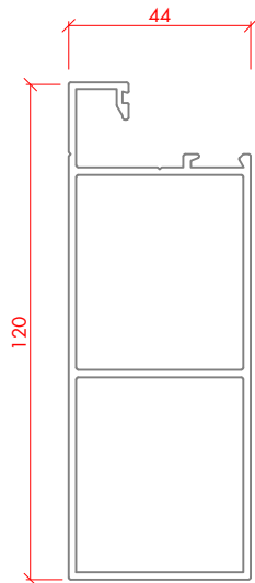
BOTTOM GLAZING BAR PSL 680
