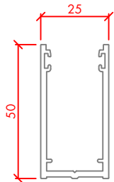
GLAZING CHANNEL PSL 542
