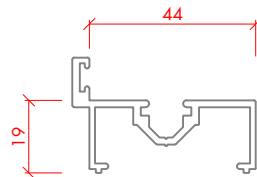
GLAZING MULLION PSL 225
