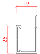
GIB LINING CAP PSL 325
