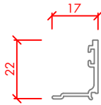
GLAZING BEAD PSL 541
