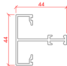
GLAZING MULLION PSL 225
