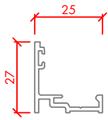
GLAZING BAR PSL 540
