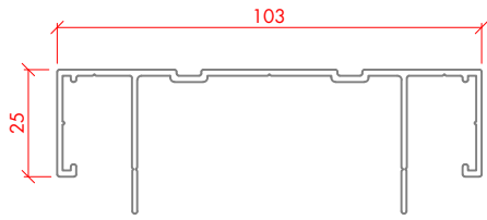
64mm GROOVED HEADSECTION PSL 400
